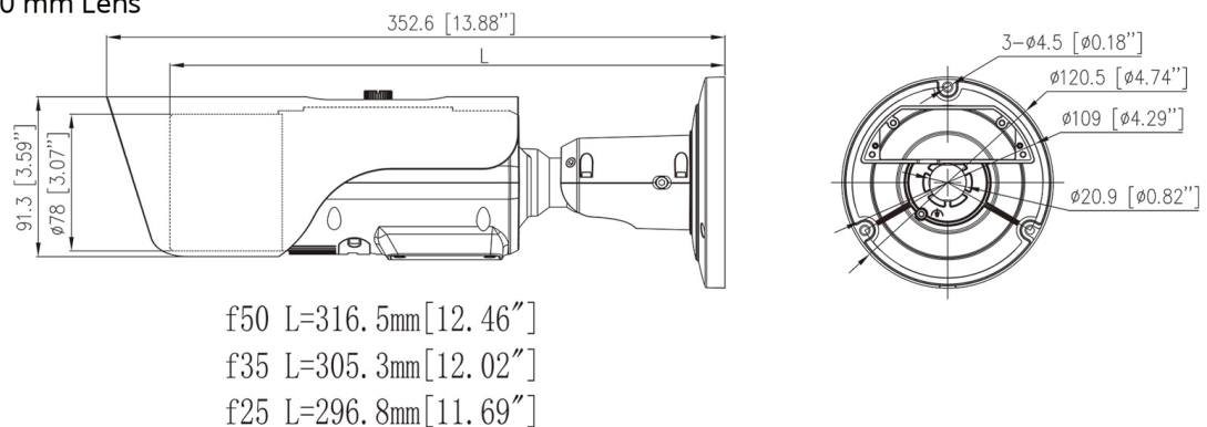
F25 / F35 / F50 mm Lens
