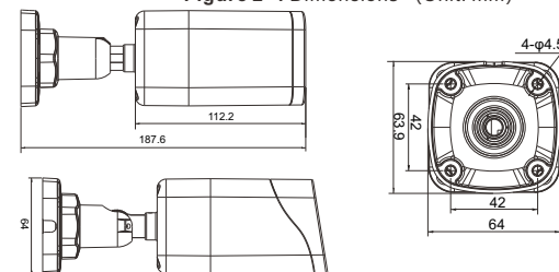
Figure 2-4 Dimensions (Unit: mm)
